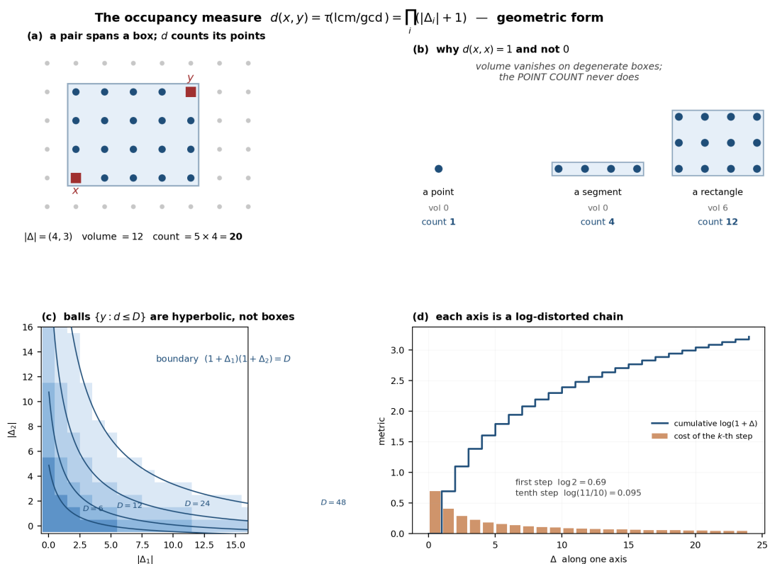
Figure 4.1. The occupancy measure. d(x, y) counts cells in the interval between two points, and equals \tau(\text{lcm}/\gcd) of their prime encodings. Balls are hyperbolic; \log d is an ordinary \ell^1 metric; and d(x, x) = 1 because a point counts itself.
