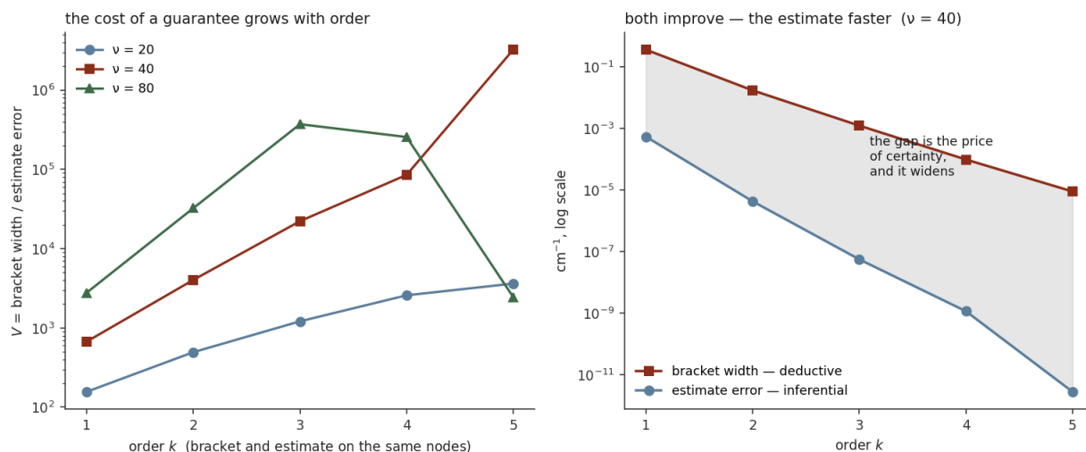
Figure 16.3. Left: V on the same node set at each order — it grows steeply, from 157 to 3.2 \times 10^6 . Right: at v = 40 both the bracket and the estimate improve as nodes are added, and the estimate improves faster; the shaded gap is the price of certainty, and it widens. An earlier version of this figure drew a floor at V = 2 through data reaching 0.24, and is withdrawn at correction 97.
