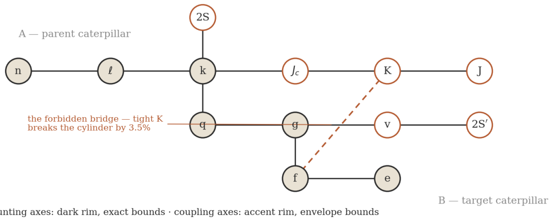
Figure 7.4. The constraint tree of the full tower: two caterpillars glued at k-q, counting axes rimmed dark (exact bounds), coupling axes in the accent (envelopes) — the Chapter 7 dichotomy drawn — with the forbidden f...K bridge dashed and priced at 3.5%.
